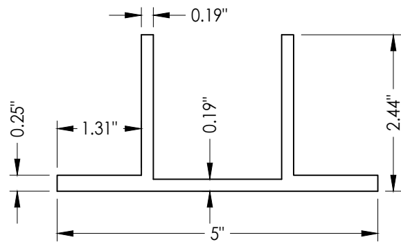
G BRAC-1 SADDLE CLIP 2" wide
